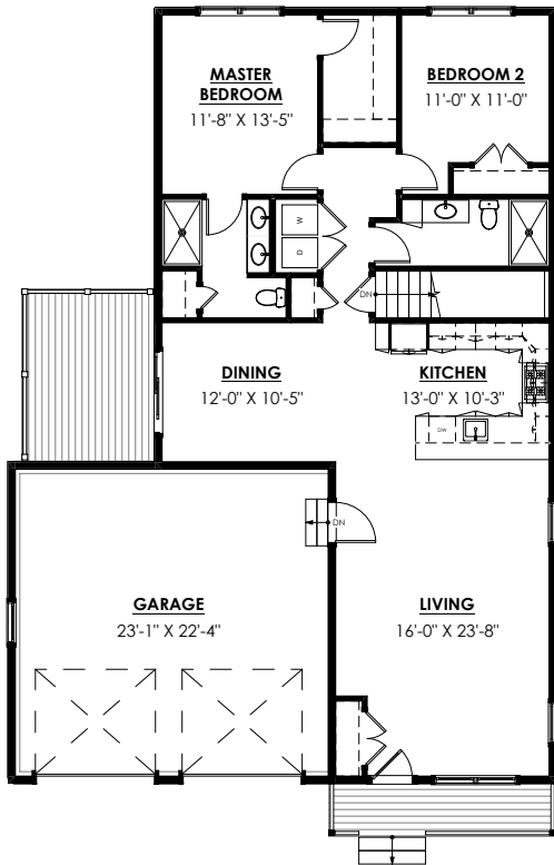
FIRST LEVEL CEILING HEIGHT = 9'-0"
